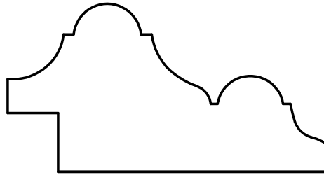
W-3285 1-1/4" x 2-3/8" 3/8" x 7/16" Rabbet
