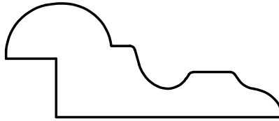
W-2253 7/8" x 2-1/16" 3/8" x 7/16" Rabbet
