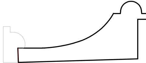
W-2871 1-1/16'' \times 2-1/4'' 1/4'' \times 11/16'' Rabbet Accepts 11/16'' - 3/4'' material (goes with W-2870)
