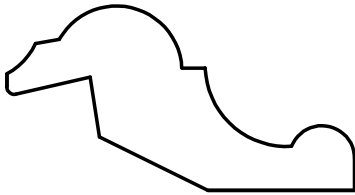
W-3270 11/16" x 1.894" 7/16" x 1/2" Rabbet Accepts 1/2" material
