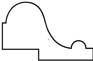
W-3663 1" x 1-9/16" 3/16" x 5/8" Rabbet
