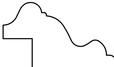
W-688 1-1/8" x 1-15/16" 1/2" x 1/2" Rabbet
