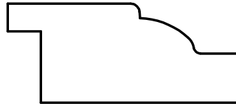
W-3239 3/4" x 1-3/4" 1/4" x 1/2" Rabbet
