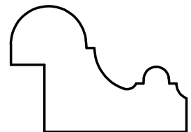
W-3420 15/16" x 1-5/16" 1/4" x 1/2" Rabbet
