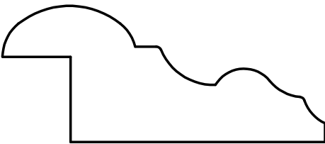
W-2206 1" x 2-3/8" 1/2" x 5/8" Rabbet
