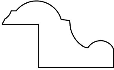
W-3759 1-1/8" x 1-15/16" Rabbet: 5/8" x 3/4"
