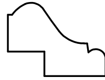
W-3258 3/4" x 1" 3/8" x 1/4" Rabbet
