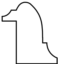
W-2787 1-1/8" x 1" 1/4" x 3/4" Rabbet
