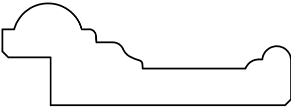
W-453 1-1/16" x 3" 1/2" x 1/2" Rabbet
