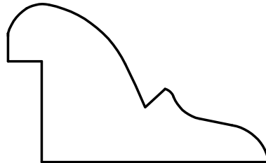
W-3080 1-3/16'' \times 1-15/16'' 1/4'' \times 3/4'' Rabbet
