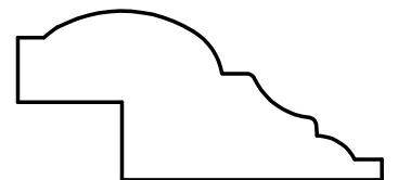
W-2462 13/16" x 1-3/4" 1/2" x 3/8" Rabbet
