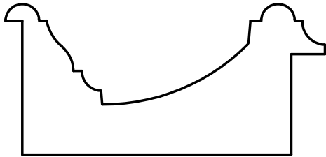
W-2961 1-1/8'' \times 2-3/8'' 1/8'' \times 1'' Rabbet 1/4'' \times 3/4'' Rabbet
