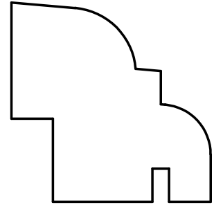
W-3304 1-1/2" x 1-1/2" 5/16" x 5/8" Rabbet
