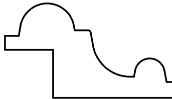
W-2595 1" x 1-3/4" 1/2" x 1/2" Rabbet
