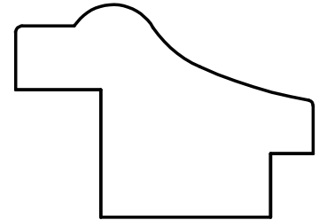
W-2584 1-1/4" x 1-3/4" 1/2" x 3/4" and 1/4" x 3/8" Rabbet
