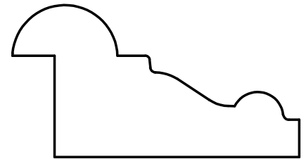
W-2213 1-1/8" x 2-1/8" 5/16" x 3/4" Rabbet
