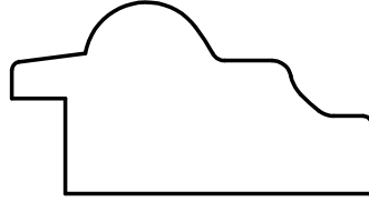
W-1952 15/16" x 1-1/16" 1/4" x 7/16" Rabbet
