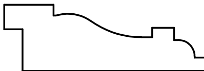
W-2412 11/16" x 2-1/16" 3/16" x 9/16" Rabbet
