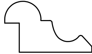
W-843 7/8" x 1-1/2" 1/4" x 1/2" Rabbet
