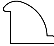
W-3763 3/4" x 7/8" Rabbet: 1/8" x 9/16"
