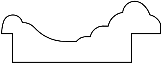
W-2839 1-1/16'' \times 2-3/4'' 3/16'' \times 1/2'' Rabbet 1/2'' \times 1/2'' Rabbet
