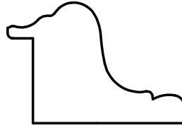
W-2011 15/16" x 1-5/16" 1/8" x 5/8" Rabbet
