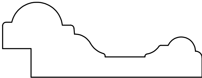
W-602 1-5/16" x 3-1/2"
