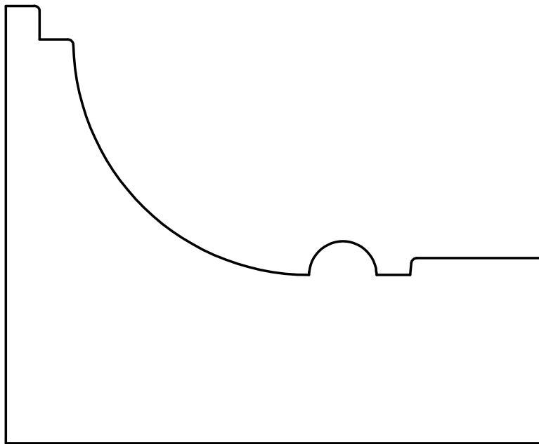
W-2092 3-1/4" x 4"
