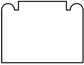
W-3372 1-1/8" x 1-1/2"
