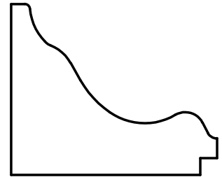
W-2040 1-1/4" x 1-9/16"
