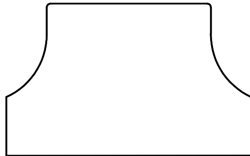
W-3106 1-5/8" x 2-5/8"
