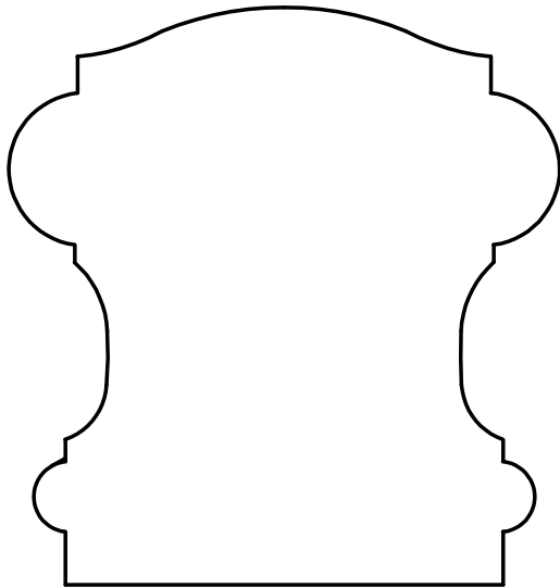
W-3485 2-5/8" x 2-3/4"
