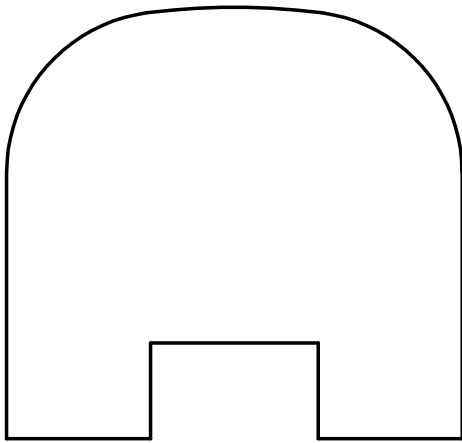
W-3048 2-1/4" x 2-3/8" 1/2" x 7/8" plow
