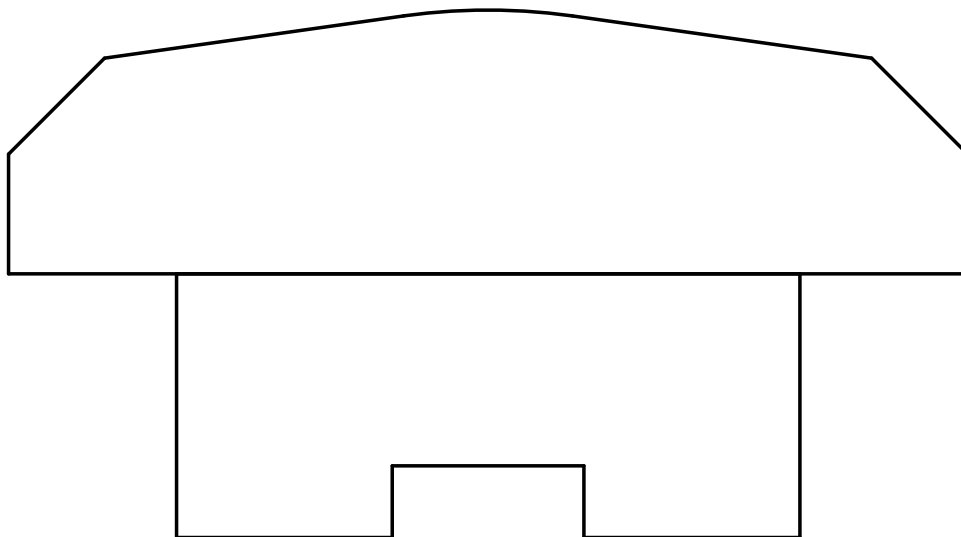
W-3631 1-3/8" x 5" 2 pc. Hand rail
