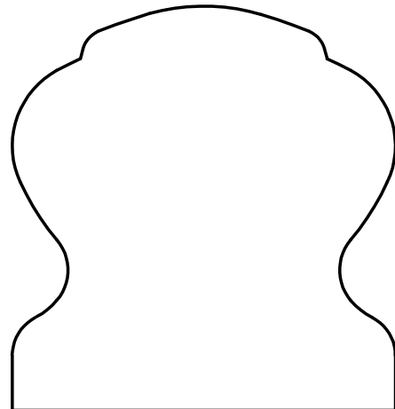
W-630M 2-3/8" x 2-1/4" Width can vary
