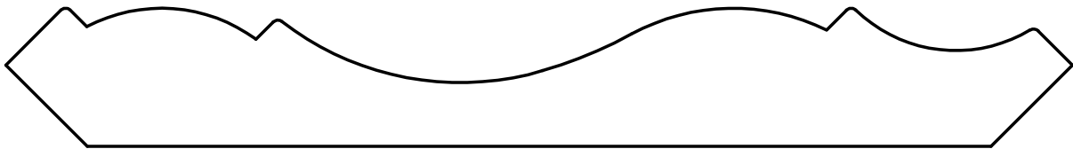
W-2441 13/16" x 5-1/4"
