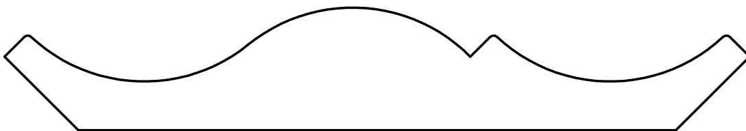
W-2162 15/16" x 5-11/16"
