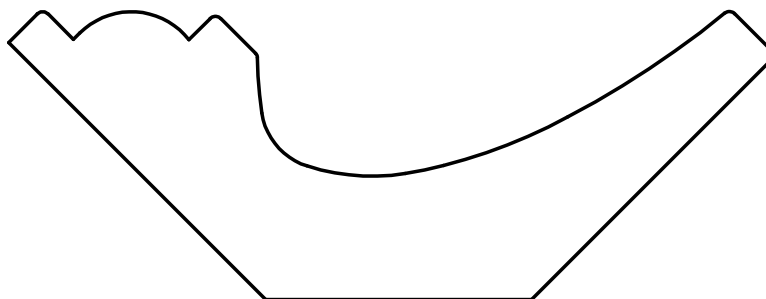
W-3152 1-1/2" x 4"
