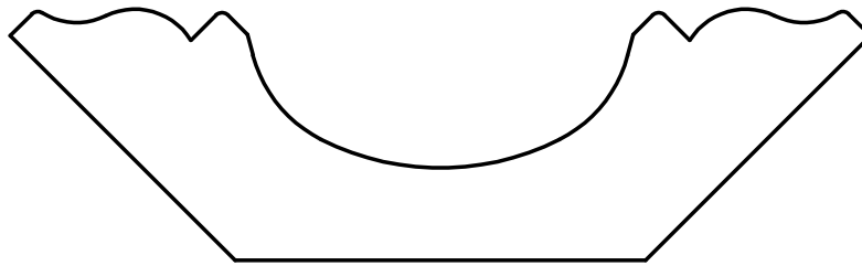
W-418 1-3/16" x 4-1/16"
