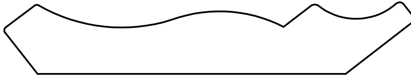
W-2928 3/4" x 4-1/4"
