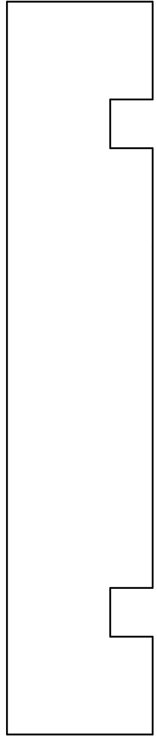
W-2629 1-1/2" x 7-1/2"
