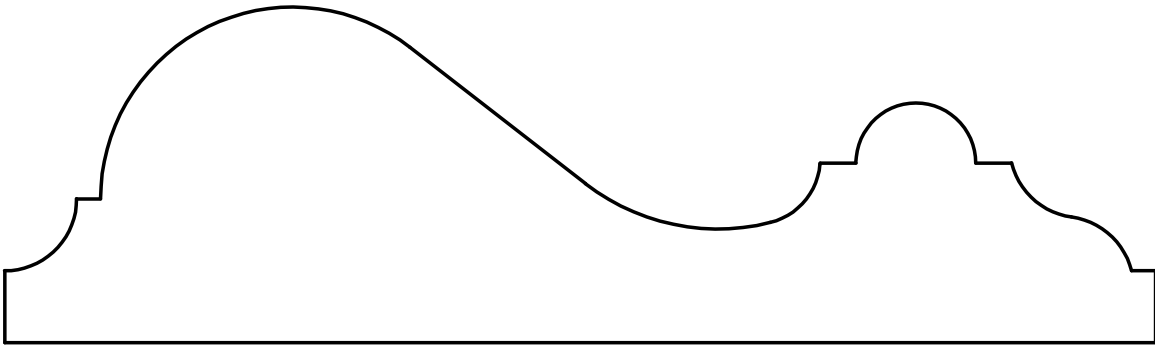
W-1252 1-3/4" x 6"
