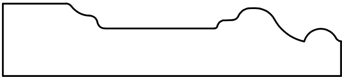
W-1034 3/4" x 3-1/2"
