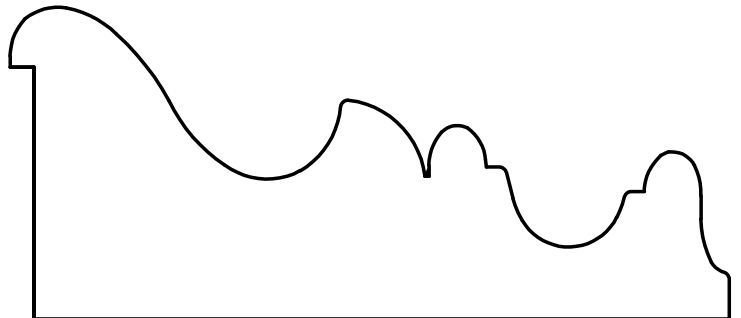
W-2859 1-5/8" x 3-3/4" Rabbit: 1/8" x 1-5/16" (goes with W-2860 & W-2861)
