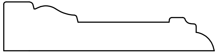
W-244 13/16" x 3-1/2"
