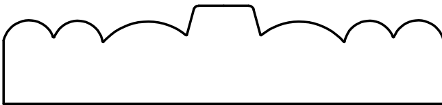
W-2571 3/4" x 3.348"
