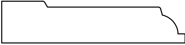
W-580 3/4" x 3-1/4"
