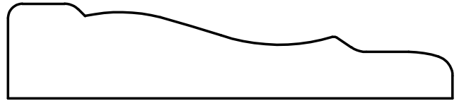
W-1924 11/16" x 3-1/4"
