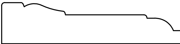
W-263 3/4" x 3-1/4"
