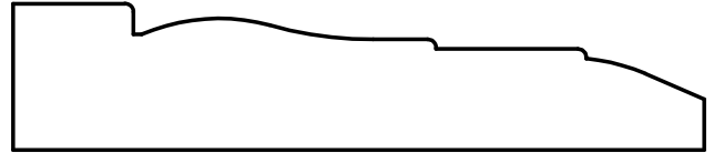
W-420 11/16" x 3-1/4"
