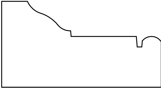
W-2847 1-3/4" x 3-1/4"
