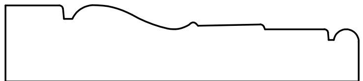
W-859 13/16" x 3-3/4"
