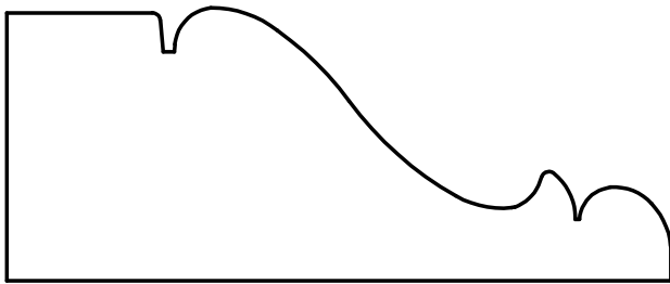
W-2858 1-5/16" x 3-3/16"
