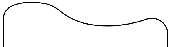
W-2674 13/16" x 2-31/32"
