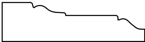
W-727 11/16" x 2-1/2"
