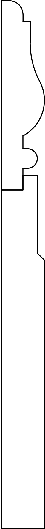
W-1603 3/4" x 10-3/4" *BOTTOM NOT FULL SIZE
