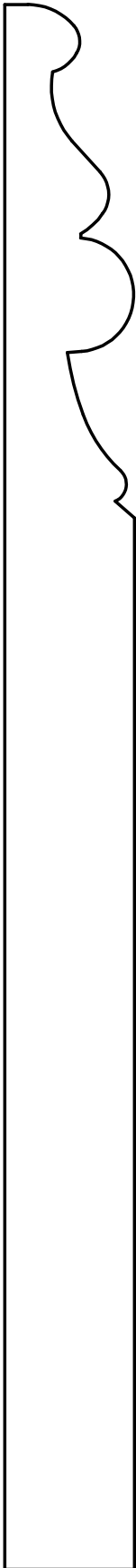
W-3182 shown at 3/4" x 9" (can be run up to 11-1/16")
