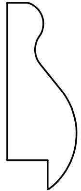
W-748 3/4" x 2" Rabbit: 5/16" x 7/16"
