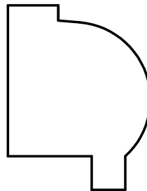
W-1858 1-1/16" x 1-3/8" Rabbit: 1/4" x 5/8"
