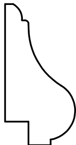
W-694 3/4" x 1-1/2" Rabbit: 1/4" x 1/4"
