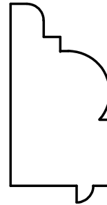
W-3227 3/4" \times 1-1/2" Rabbet: 1/8" \times 1/2"
