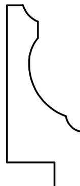
W-2804 13/16" x 1-7/8" Rabbet: 1/4" x 1/2"
