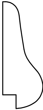
W-1468 3/4" x 2" Rabbit: 1/4" x 1/4"
