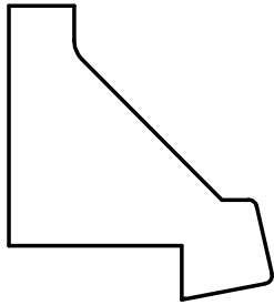
W-1450 1-1/4" x 1-3/8" Rabbit: 1/4" x 13/16"
