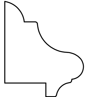
W-1171 1-7/16" x 1-3/4" Rabbit: 1/4" x 3/4"
