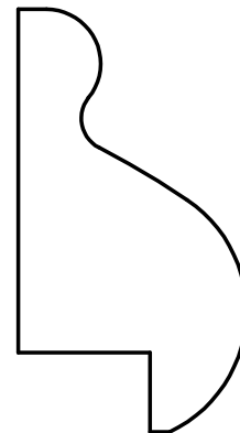
W-747 1-1/16" x 2" Rabbit: 3/8" x 5/8"
