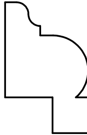
W-3216 7/8" \times 1-3/8" Rabbet: 1/2" \times 3/4"
