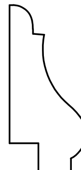
W-3029 7/8" x 1-13/16" Rabbet: 5/16" x 5/16"
