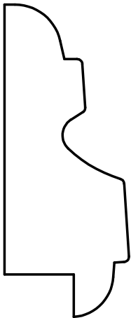
W-1673 15/16" x 2-5/16" Rabbit: 5/16" x 1/2"
