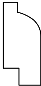
W-3542 11/16" \times 1-1/2" Rabbet: 9/32" \times 5/16"
