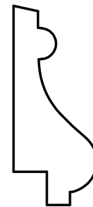
W-523 5/8" x 1-1/2" Rabbit: 1/4" x 1/4"
