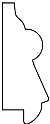
W-644 13/16" x 2-1/8" Rabbit: 1/4" x 3/8"
