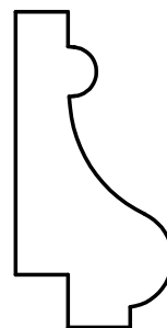
W-2510 3/4" x 1-1/2" Rabbet: 1/4" x 1/4"
