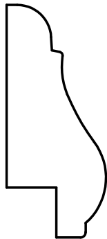
W-288 3/4" x 1-3/4" Rabbit: 3/8" x 3/8"
