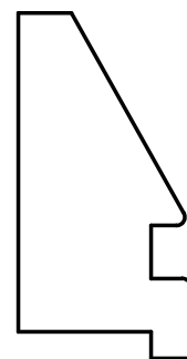
W-2523 13/16" x 1-5/8" Rabbet: 1/8" x 5/8"
