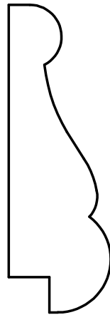
W-405 3/4" x 2-1/4" Rabbit: 1/4" x 5/16"
