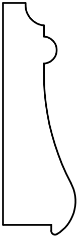
W-3061 3/4" \times 2-3/8" Rabbet: 3/32" \times 1/2"
