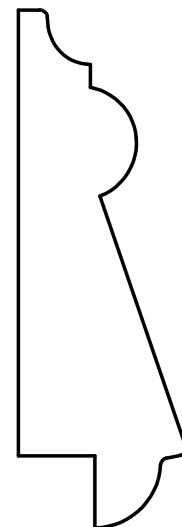
W-1927 7/8" x 2-11/16" Rabbit: 3/8" x 3/8"
