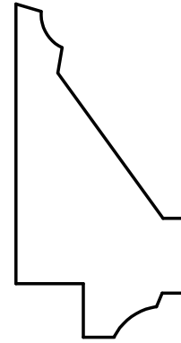
W-1447 1" x 2" Rabbit: 5/16" x 3/8"
