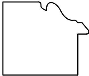
W-2546 1-1/4" x 1-1/2" * 3/16" x 0.70" RABBET
