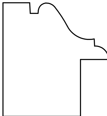
W-1087 2" x 1-7/8" * 1/2" x 1"
