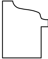
W-3581 1" x 1-1/4" Rabbet: 3/32" x 11/16"
