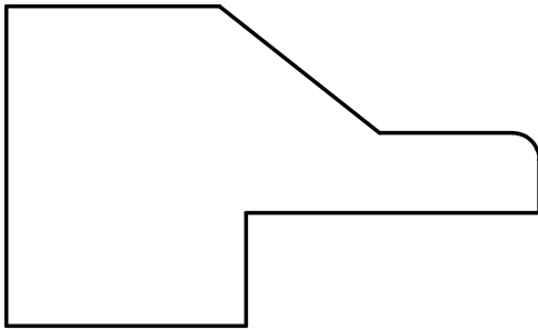
W-1424 1-1/2" x 2-1/2" * 1/2" x 1-3/8" RABBET
