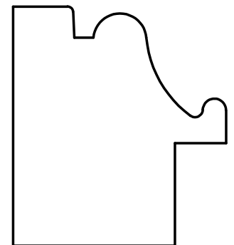
W-1090 1-3/4" x 1-9/16" * 3/8" x 3/4" RABBET
