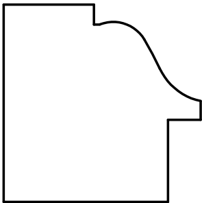
W-833 1-1/2" x 1-1/2" * 1/4" x 5/8" RABBET
