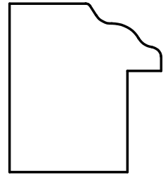
W-1850 1-1/4" x 1-1/8" * 1/4" x 3/4" RABBET
