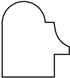
W-2492 1-1/4" x 1-1/8" * 1/4" x 3/8" RABBET
