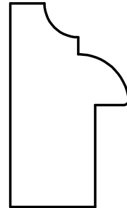
W-3347 7/8" x 1-1/2" Rabbet: 1/4" x 3/4"
