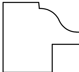
W-3682 1-1/4" x 1-3/8" Rabbet: 1/2" x 1/2"
