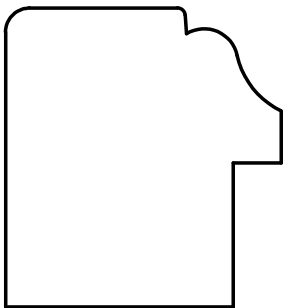
W-1449 1-9/16" x 1-7/16" * 1/4" x 3/4" RABBET
