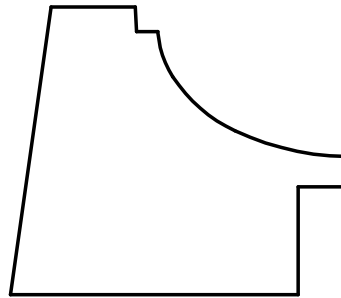
W-3651 1-1/2" x 1-3/4" Rabbet: 1/4" x 9/16"
