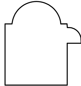
W-2825 1-1/2" x 1-3/8" Rabbet: 1/4" x 3/4"
