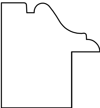
W-2149 1-7/8" x 1-3/4" * 1/2" x 1" RABBET
