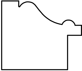
W-1109 1-1/4" x 1-7/16" * 1/4" x 5/8" RABBET
