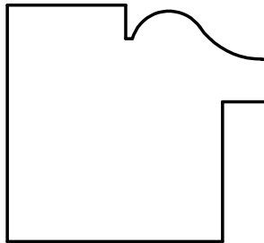
W-860 1-3/8" x 1-1/2" * 1/4" x 13/16" RABBET
