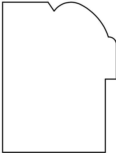
W-2003 2-9/16" x 1-15/16" * 3/16" x 1 1/4" RABBET
