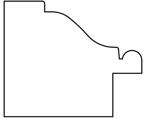
W-793 2" x 2-3/8" * 1/2" x 3/4" RABBET
