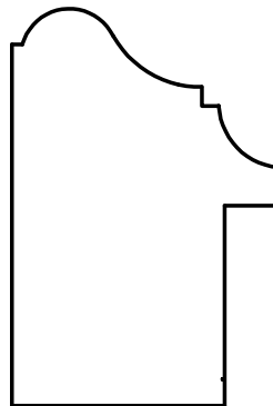
W-2785 1-7/8" x 1-1/4" Rabbet: 1/4" x 15/16"
