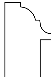
W-3784 1" x 1-5/8" Rabbet: 1/4" x 13/16"
