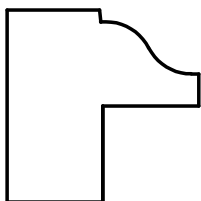
W-3675 1" x 1" Rabbet: 1/2" x 1/2"
