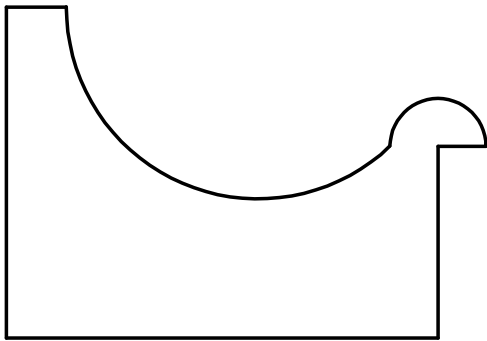
W-3108 1-23/32" x 2-1/2" Rabbet: 1/4" x 1"
