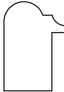
W-1742 1-5/8" x 1-1/8" * 1/4" x 1-1/16" RABBET
