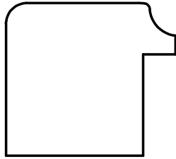
W-1321 1-1/8" x 1-1/4" * 1/4" x 3/4" RABBET
