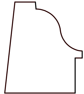
W-3671 1-5/8" x 1-3/8" Rabbet: 1/8" x 5/8"
