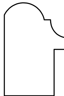
W-3560 1-1/16" x 1-5/8" Rabbet: 3/16" x 13/16"
