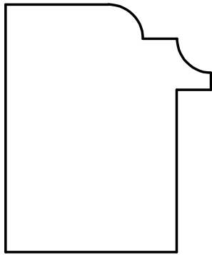
W-3245 1-1/2" x 1-13/16" Rabbet: 1/4" x 1-3/16"
