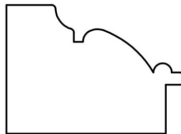
W-2283A 1-5/16" x 1-13/16" * 3/16" x 1/2" RABBET
