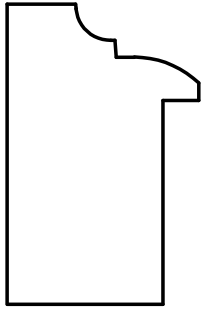
W-3566 1" x 1-5/16" Rabbet: 3/6" x 1-1/16"
