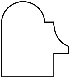
W-2492 1-1/4" x 1-1/8" * 1/4" x 3/8" RABBET
