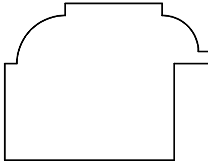
W-2678 1-5/8" x 2-1/8" 3/8" x 1" RABBET
